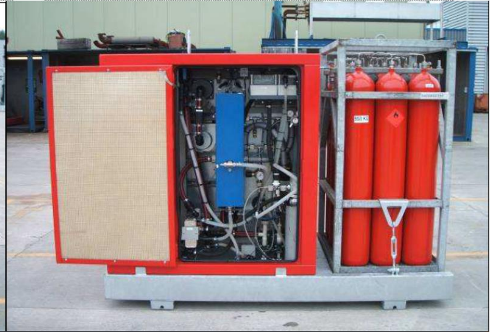
Process Side of the Canopy
